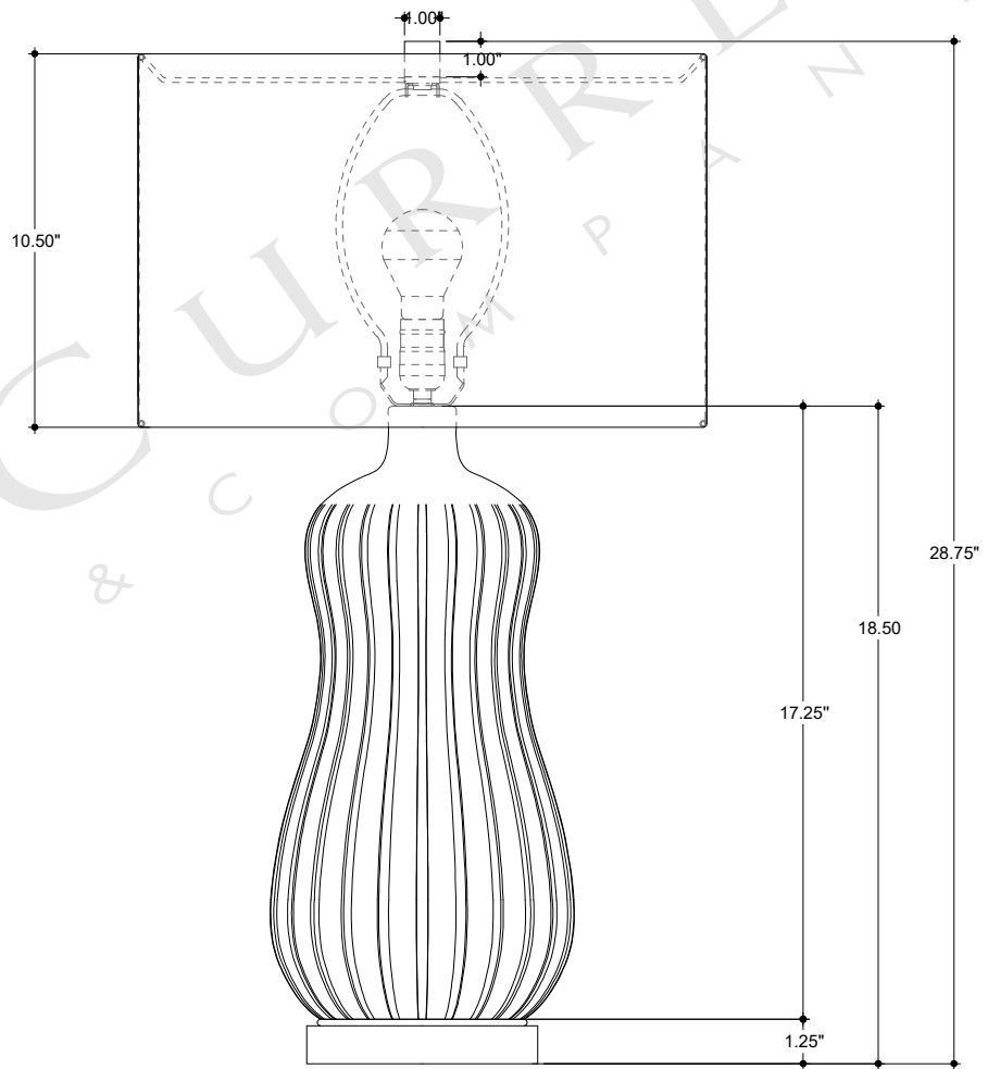
FRONT VIEW
